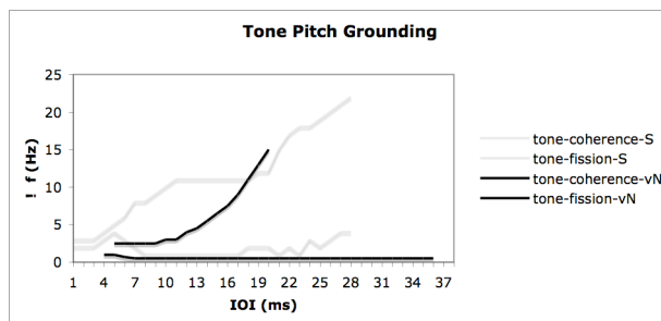
Figure 4: Tone Pitch Grounding
